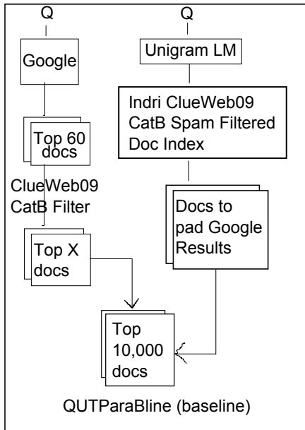
Figure 1: Baseline: QUTParaBline.
