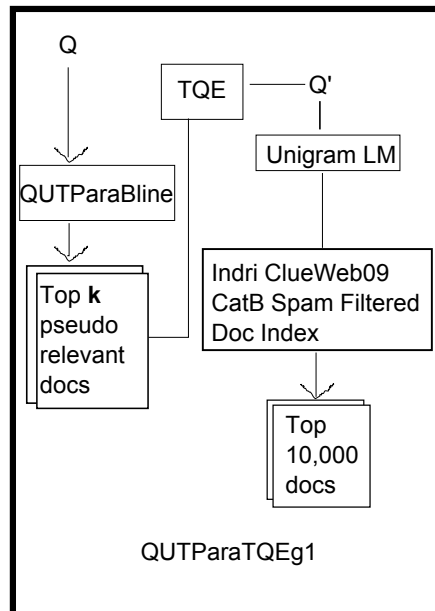
Figure 2: QUTParaTQ Eg1.
